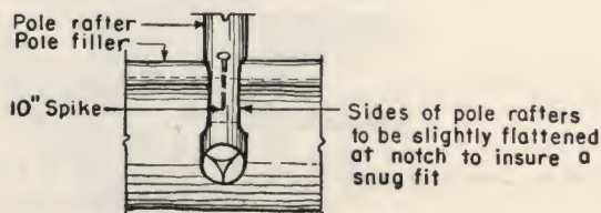
NOTCHED POLE RAFTERS
