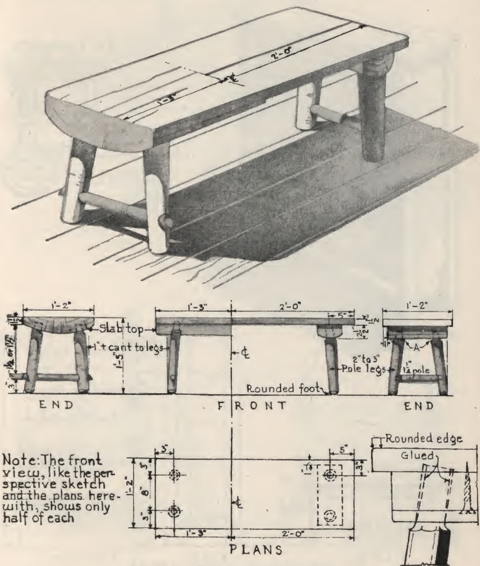
FIGURE 45.—Plan for making benches.
