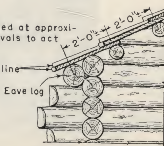
EAVE SECTIONS
