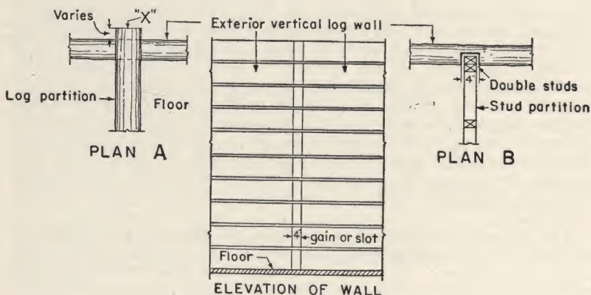
FIGURE 22.—Interior partitions.
