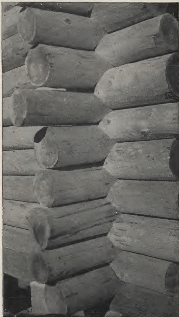
FIGURE 2.—The round-notch or saddle corner. This is an unusually fine example of scribing and fitting logs together. The square-cut logs have yet to be dressed and shaped with the ax to give them a pleasing appearance.
