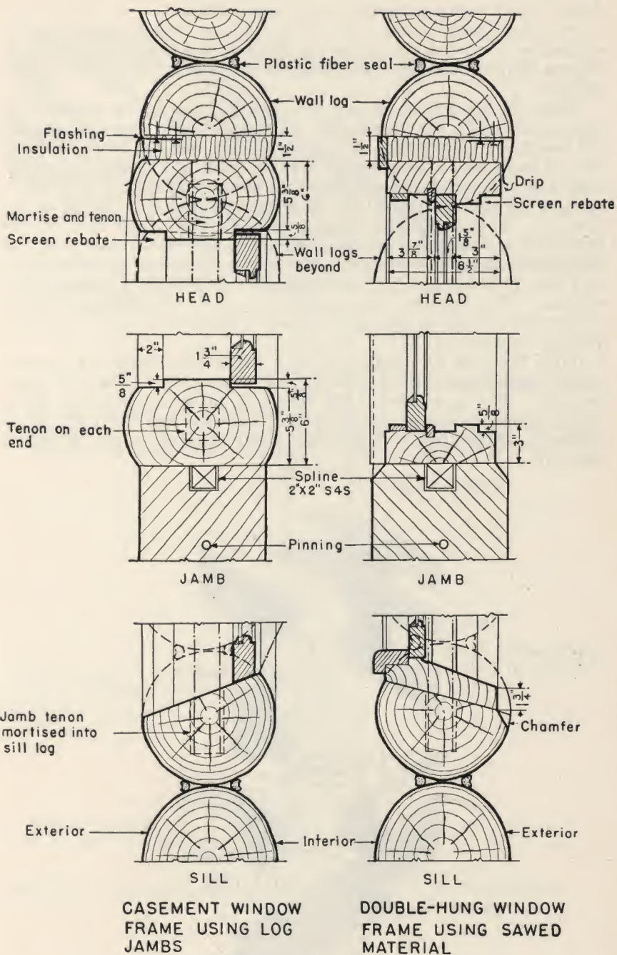
FIGURE 15.—Window frames.
