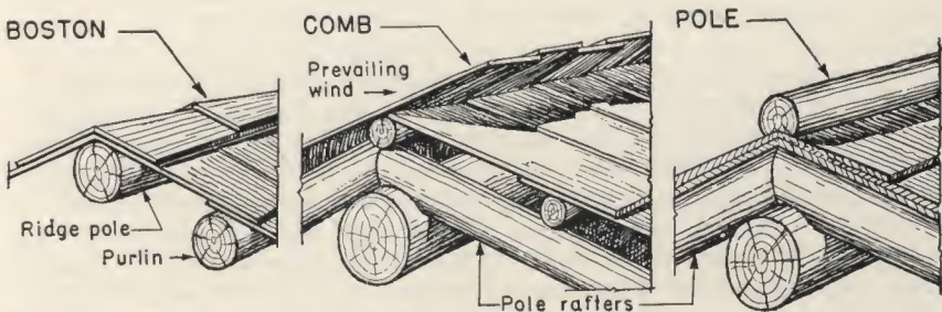
FIGURE 21.—Ridge treatments.
