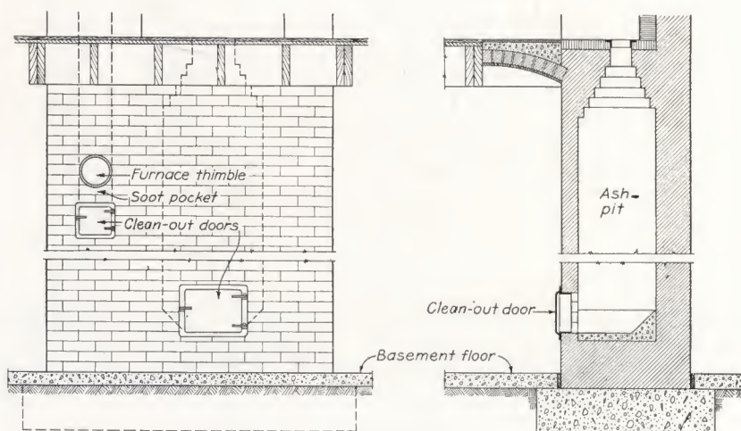
FIGURE 35.—The ashpit should be of tight masonry and should be provided with a tightly fitting iron clean-out door and frame about 10 by 12 inches in size. A clean-out for the furnace flue as shown is sometimes provided.
