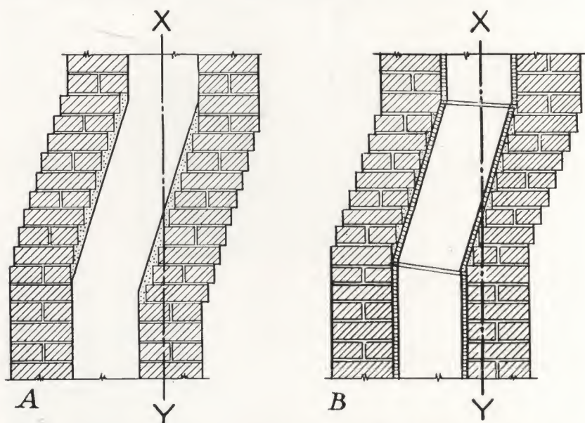
FIGURE 8.—For structural safety the amount of offset must be limited so that the center line, XY , of the upper flue will not fall beyond the center of the wall of the lower flue. A , Offsetting of the left wall of an unlined flue is started two brick courses higher than on the right wall so that the area of the sloping section will not be reduced after plastering; B , a lined flue showing the method of cutting the tile.
