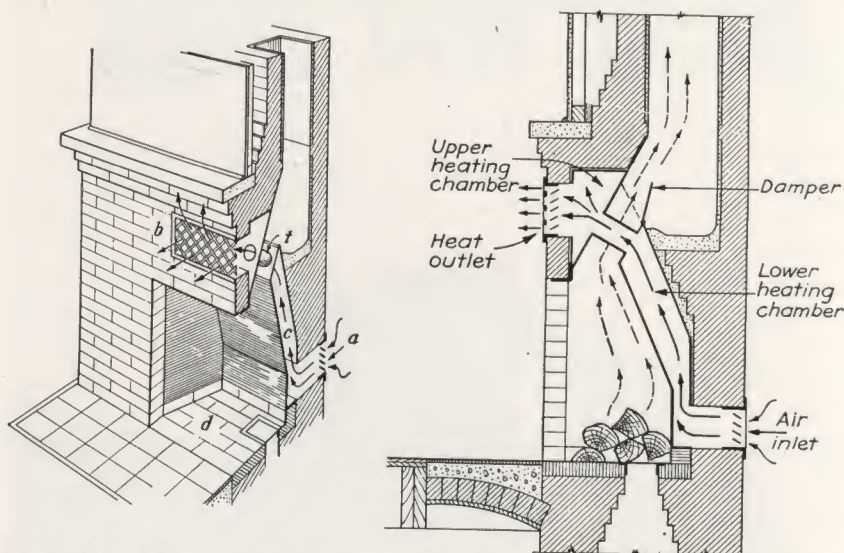
FIGURE 20.—In this modified fireplace air enters the inlet, a , from outside and is heated as it rises by natural circulation through the back chamber, c , and the tubes, t , being discharged into the room from the register, b . Air for supporting combustion is drawn into the fire at d and passes between the tubes up the flue. A damper is also provided to close the air inlet.
