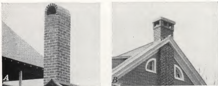
FIGURE 18.—A, A common type of arched hood; B, flat stone hood; note the vithe separating the two flues.
