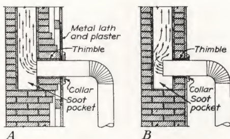
FIGURE 12.— A , Connection to chimney where furring is used. The brick are built out around the thimble as a protection against its cracking. This is a fire hazard that is frequently overlooked. B , Connection when plaster is applied directly to the masonry. Note that the pipe extends too far into the flue. It should be as shown in A .
